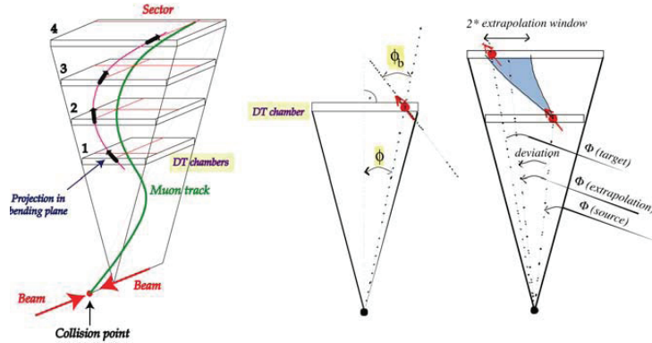
Figure 7.9: DTTF extrapolation scheme
