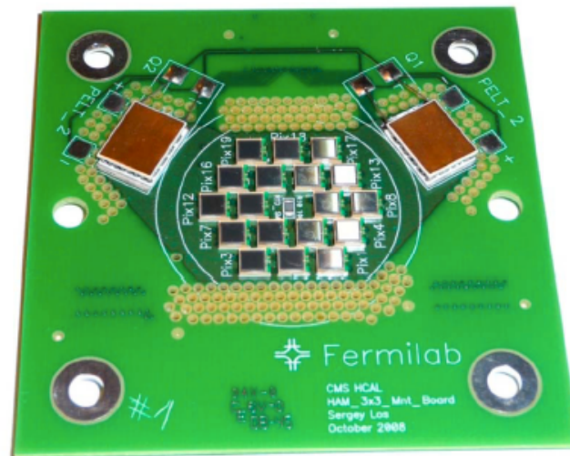
Figure 4.5: SiPM Mounting card. The larger rectangles are the 2 Peltier coolers. Also seen is a grid of 18 SiPMs with the same placement as the HPD pixels.
